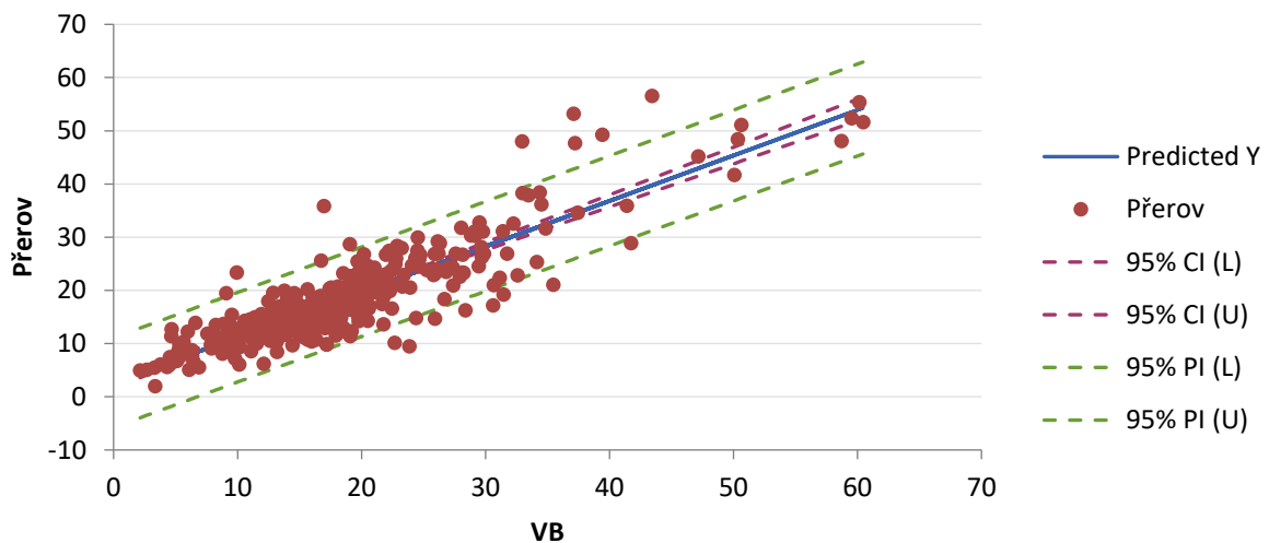
Scatter plot "Přerov" vs. "VB"
