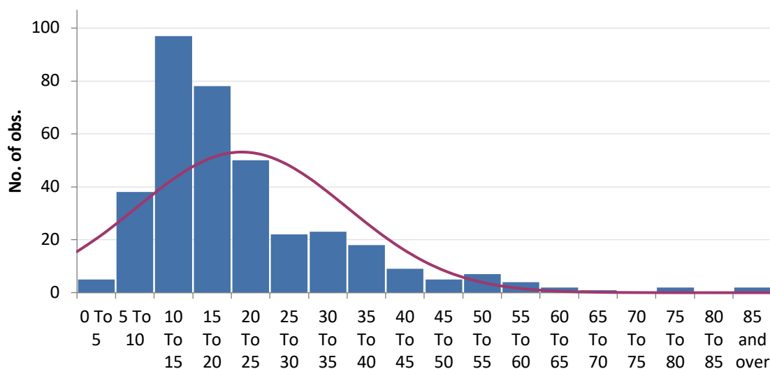
Histogram for "Olomouc Hejčín"
