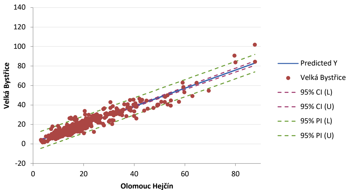
Scatter plot "Velká Bystřice" vs. "Olomouc Hejčín"
